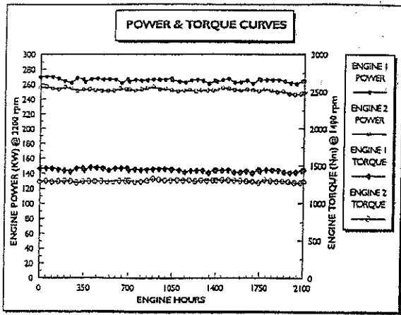
Figure 4 - Engine Power and Torque Comparison.
