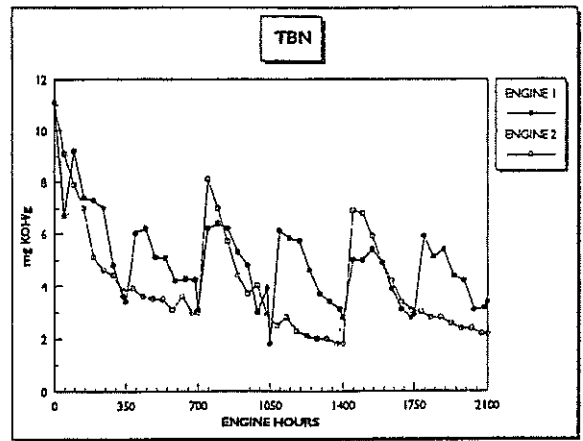
Figure 10 - TBN.
