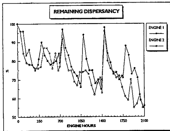
Figure 9 - Remaining Dispersancy.
