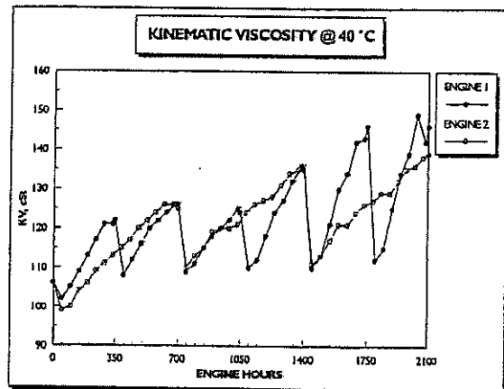
Figure 7 - Oil Viscosity.
