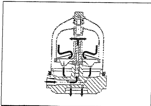
Figure 2 - Principle of operation for a bypass oil cleaning centrifuge.
