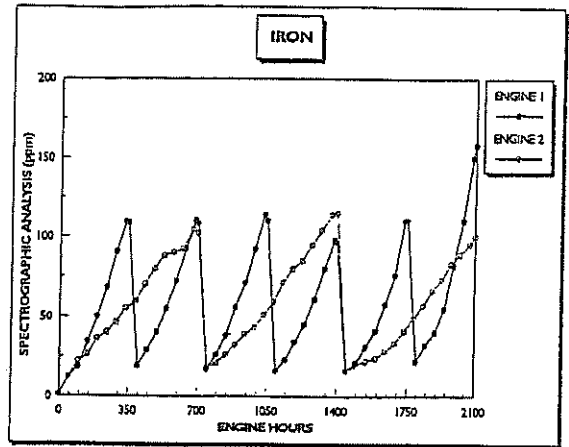
Figure 6 - Spectrographic Oil Analysis of Iron in Lubricating Oil for Both Engines.
