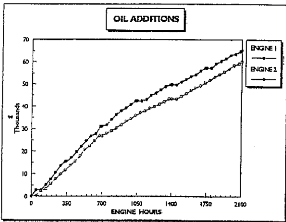
Figure 5 - Cumulative Oil Additions for Both Engines.
