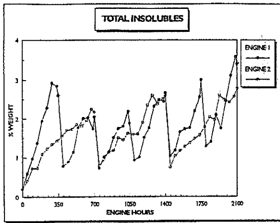
Figure 8 - Total Insolubles.
